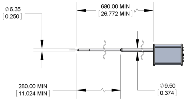
Plasma probe with built-in RF filter
