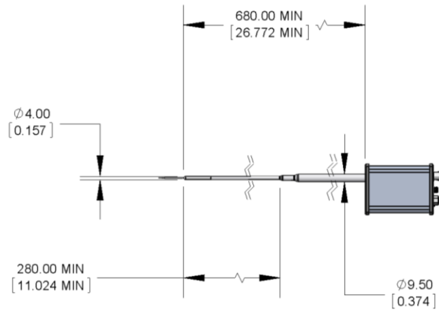
Plasma probe for DC and afterglow measurements
