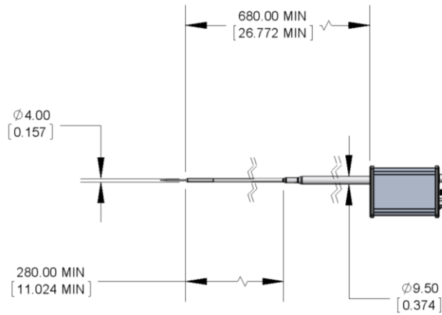
Plasma probe for DC and afterglow measurements
