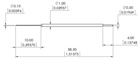
Replaceable probe tip
